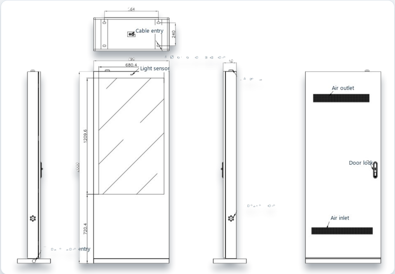
Overall 790 × 2000 × 140 mm (W × H × D); screen area 1209.6 × 680.4 mm.
